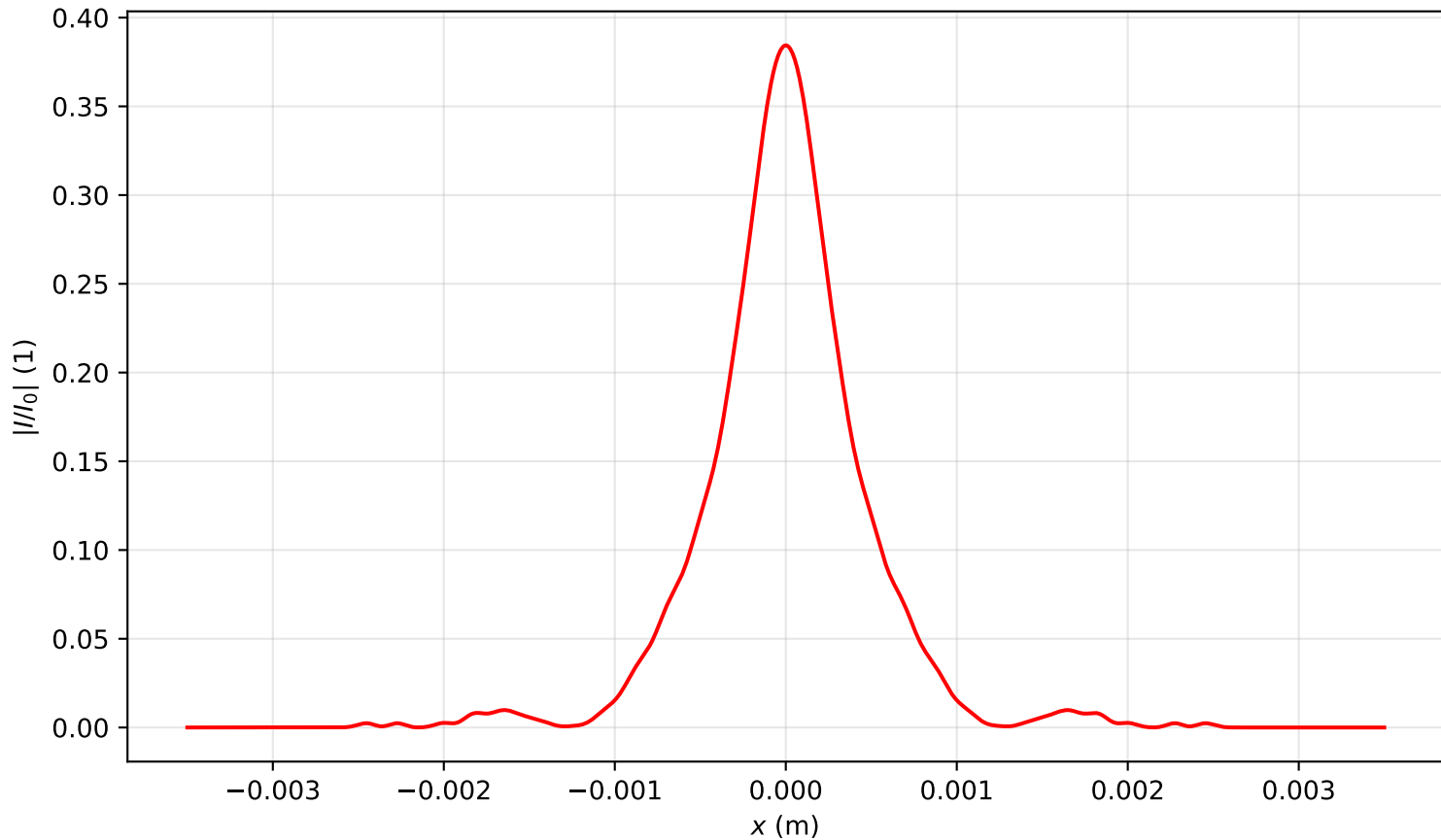
Intensity profile I(x, y = 0, z = 1.274)/I_0 , P_{in}=3.0P_{cr} , artificial time
